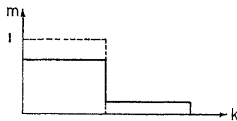
FIG. 6. Schematic distribution of holes in reciprocal space with (drawn out) and without (dotted) correlation.
