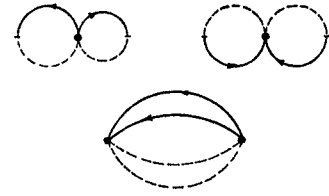
FIG. 7. Diagrams contributing to the properly correlated part of \rho_2 in the second order of density.
